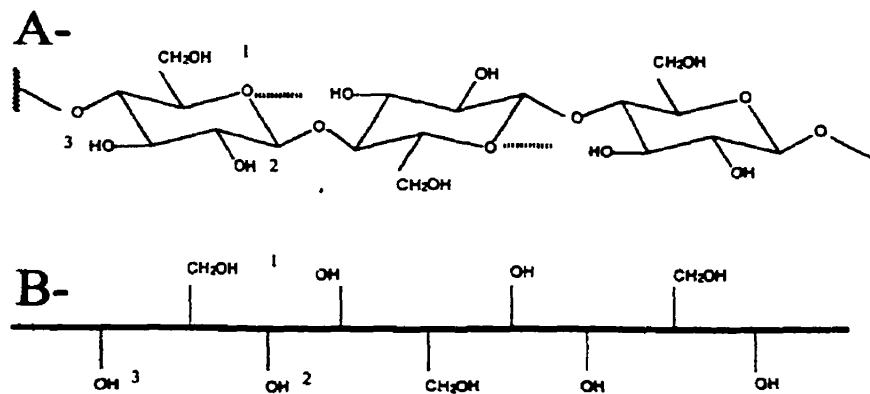
Fig. 1. Cellulose: (A) Conventional 3-D structure (B) Conventional 2-D structure.
