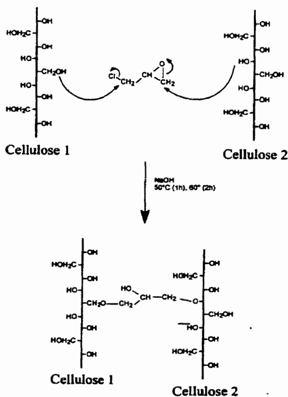
Fig. 2. Synthesis of cross-linked cellulose.
