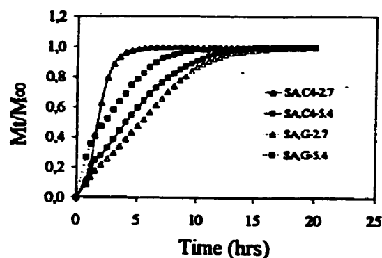
Fig. 4. Effect of OH groups attached on acetaminophen release profile.
